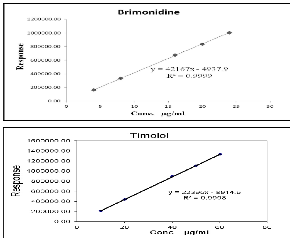
Fig.3. Calibration plot of Brimonidine Tartrate and Timolol Maleate
