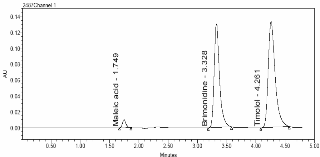
Fig.2. Typical HPLC chromatograms obtained from 20 \mu l injections of Brimonidine Tartrate (3.86 min.) and Timolol Maleate (3.86 min.) respectively under optimized chromatographic conditions.
