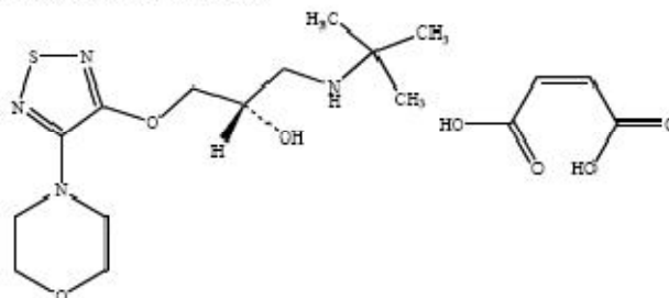
Fig.1. Structures of Brimonidine Tartrate and Timolol Maleate respectively
