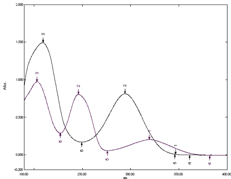
Fig.4. Typical UV spectrum of Brimonidine Tartrate and Timolol Maleate
